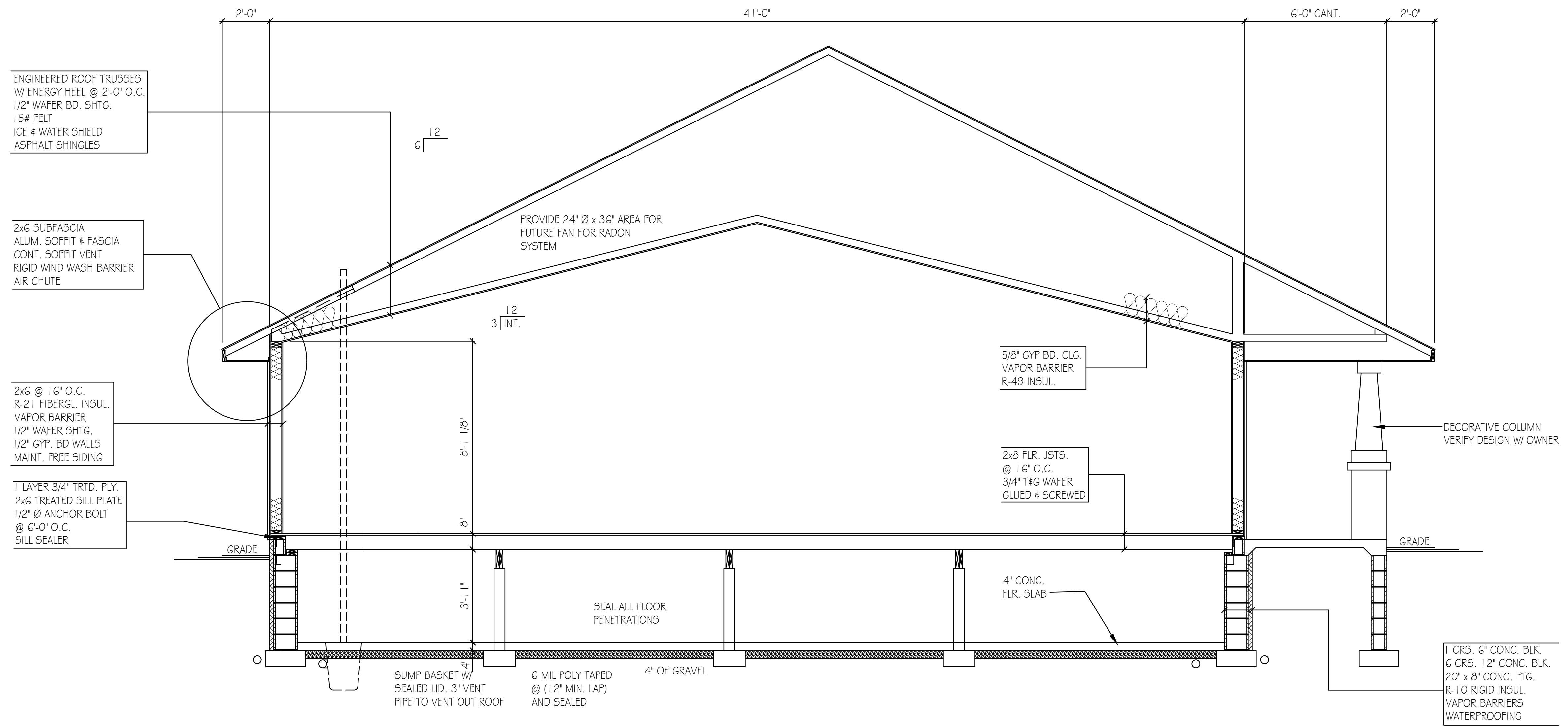
BUILDING SECTION SEE BUILDERS SPECIFICATION FOR BUILDING MATERIALS
