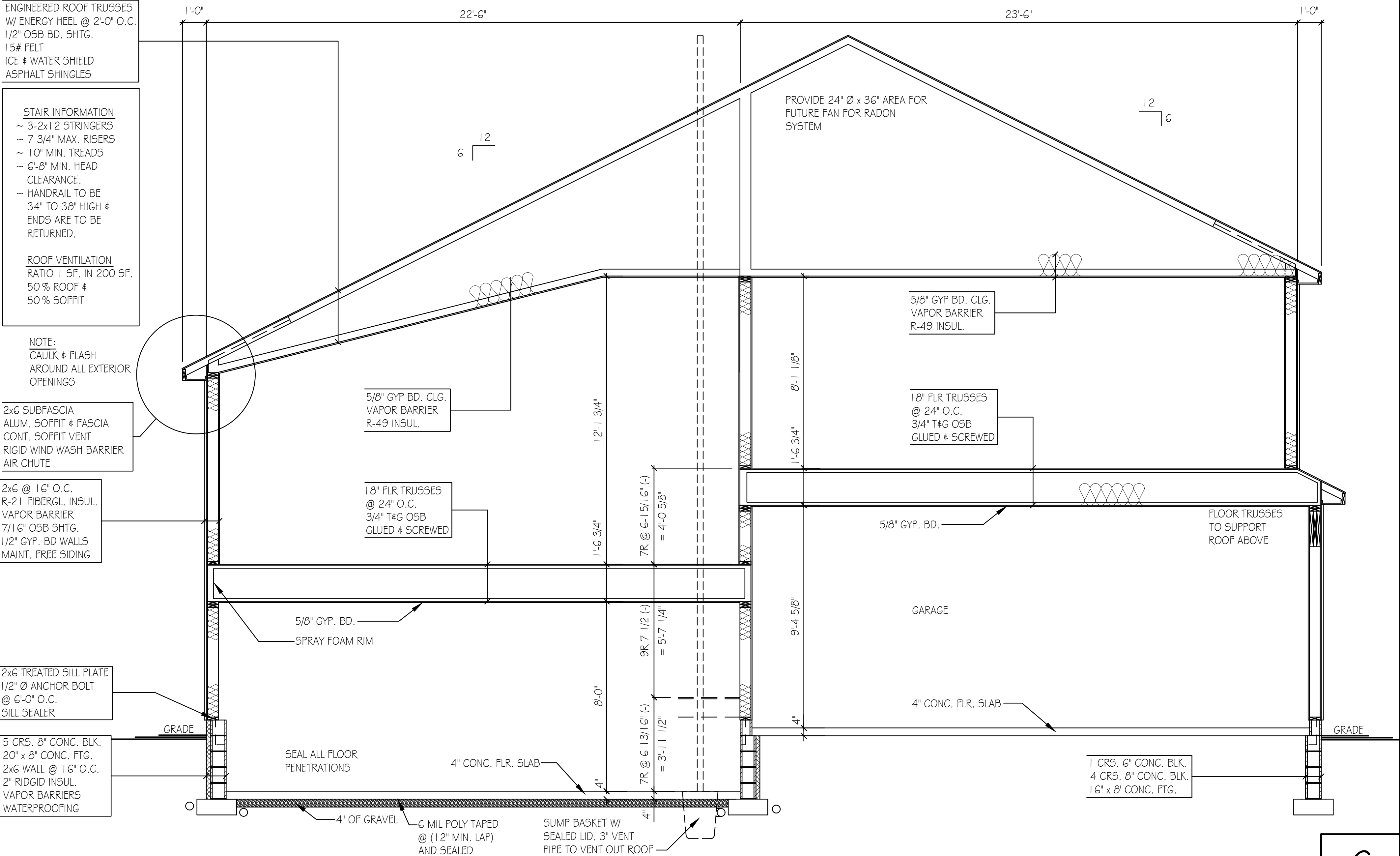
BUILDING SECTION SEE BUILDERS SPECIFICATION FOR BUILDING MATERIALS
